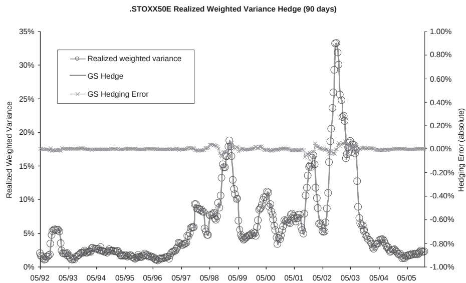
Figure A.4: Realized weighted variance versus its hedge (A.16).
