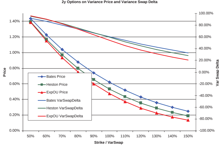
Figure 4.3: Prices and VarSwapDelta for options on variance with a 2y maturity for Fitted Heston, Fitted Bates and Fitted Exponential Ornstein-Uhlenbeck.
