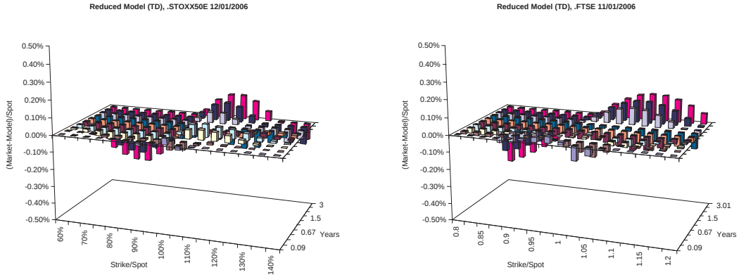
Figure 8.4: Calibration of the reduced model (8.24) with piece-wise constant VolOfVol and correlation parameters to STOXX50E and FTSE market data.
