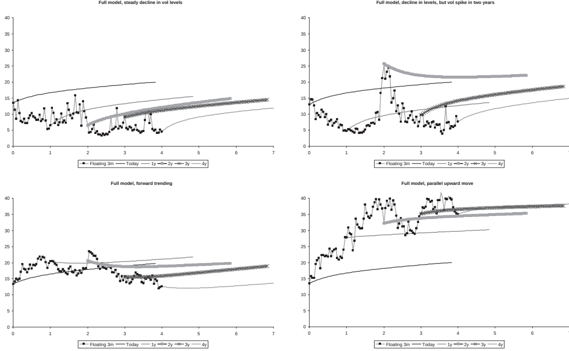
Figure 8.5: Future shapes of the variance swap curve produced by the full model. The model allows for various market scenarios, including down and upward trending volatilities. All quotes are given as “variance swap volatility”.
