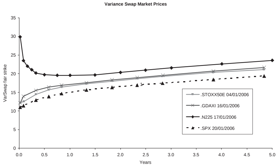
Figure 1.1: Example variance swap prices. The prices are quoted in “variance swap volatility” (1.2).
