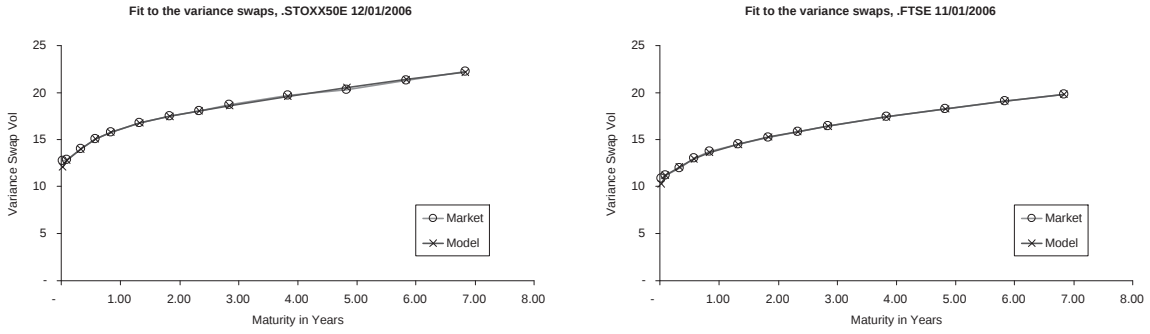
Figure 8.1: Fit of the double-mean reverting functional (7.7) to FTSE and STOXX50E market data. Note that the variance swap prices are quoted according to market standard using “variance swap volatilities”, cf. (1.2).
