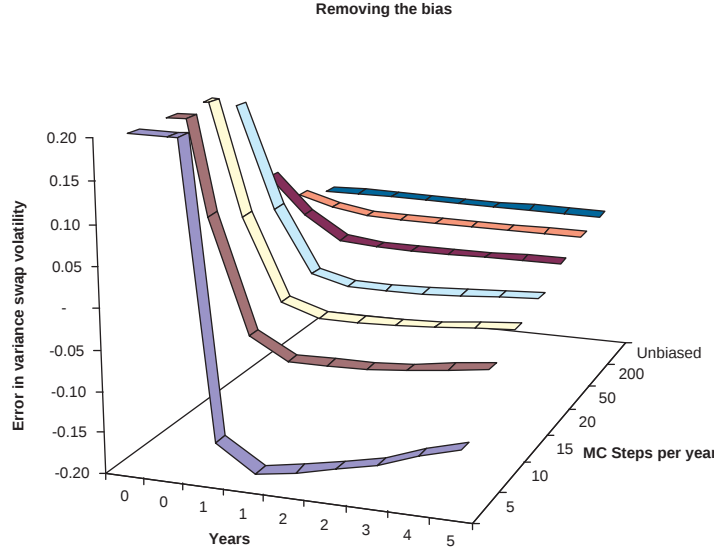
Figure 7.5: The error in variance swap volatilities \sqrt{V_0(T)/T} when used with the biased scheme (7.26). In contrast, the terminal data set (which is labeled “unbiased”) was computed using (7.29) with just one step per year.
