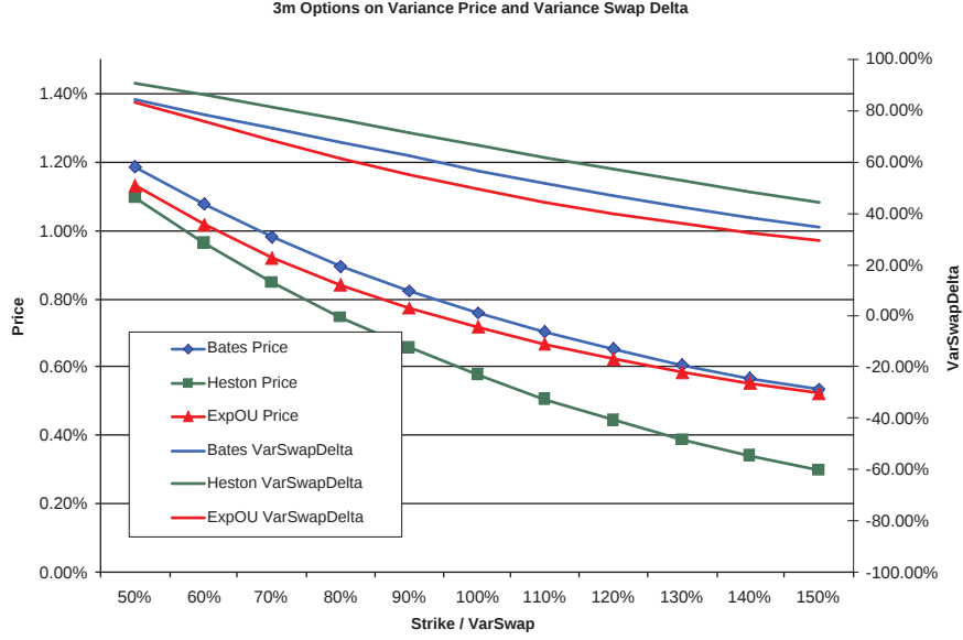
Figure 4.2: Prices and VarSwapDelta for options on variance with a 3m maturity for Fitted Heston, Fitted Bates and Fitted Exponential Ornstein-Uhlenbeck. One can clearly see the impact of not having a jump component for the Fitted Heston results.
