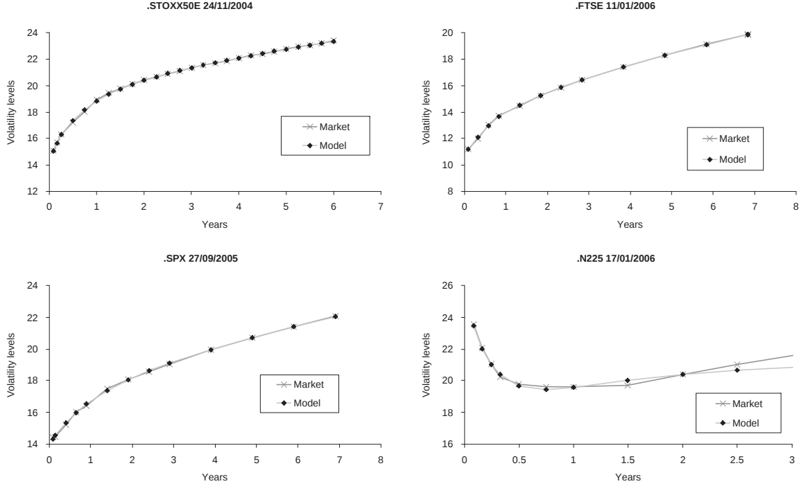
Figure 7.2: Fitting the variance curve (7.7) to market data. It generally fits well, even if the market experiences massive disruptions, as we can see in the example of the .N225 index (from Monday, January 16th 2006, to Wednesday the .N225 dropped by nearly 7% which in return drove up the prices of short term variance swaps). All graphs show “variance swap volatilities”, cf. (1.2).
