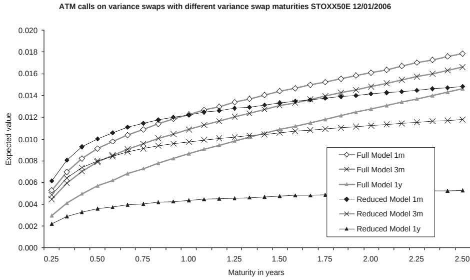
Figure 8.10: Term structures of ATM calls on variance swaps with time-to-maturity of one month, three months and one year (here, we show the expected value of (V_{T_1}(T_1, T_2) - k V_0(T_1, T_2))^+ / (T_2 - T_1) , rather than the payoff (8.25)). The discrepancy between the full and the reduced model rises as the time-to-maturity of the underlying variance swap increases. Also note the relative decline in time value for the reduced model, which is a consequence of \zeta of (8.24) converging to its invariant distribution.
