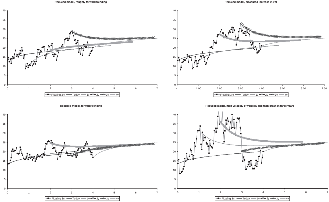
Figure 8.6: Future shapes of the variance swap curve produced by the reduced model. In comparison to figure 8.5, the long-term volatility of the variance swap curves is far more “sticky”.
