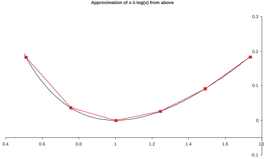
Figure A.2: Approximation of F(x) := x - \log x - 1 from above.
