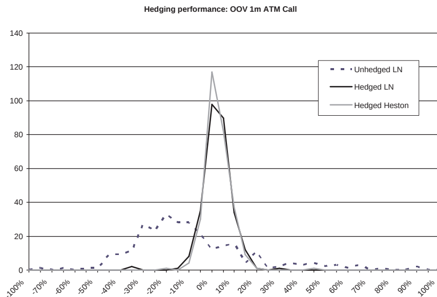
Figure 4.8: Histogram for hedging returns for 1m ATM Call on Variance. The reduction in risk is very obvious.
