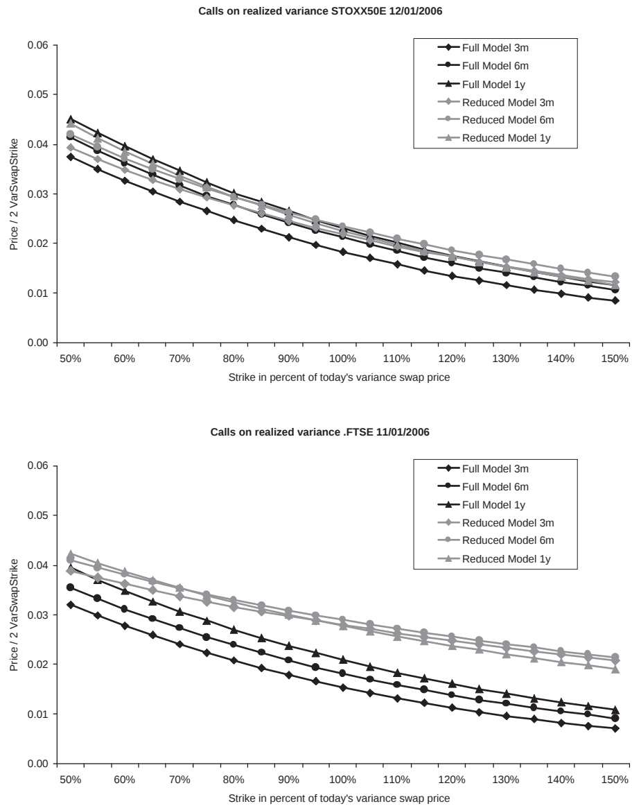
Figure 8.7: Calls on realized variance. A detailed view of the 1y call is given in figure 8.8.
