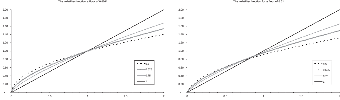
Figure 7.1: The function x \mapsto (x^+ + \epsilon)^y - \epsilon^y for a floor \epsilon of 0.0001 and 0.01.
