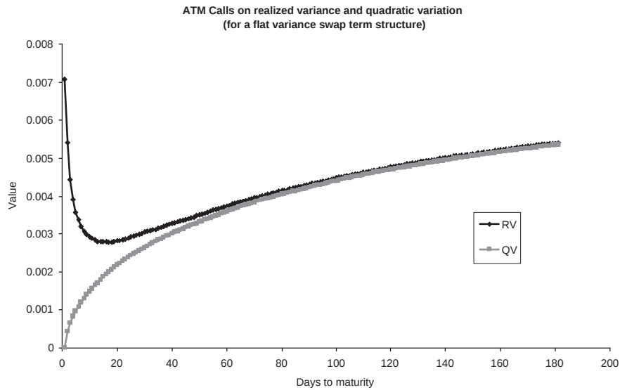
Figure 8.11: ATM calls on realized variance and quadratic variation in a Heston model with flat variance swap term structure. The graph shows that while the approximation of realized variance via quadratic variation works very well for variance swaps, it is not sufficient for non-linear payoffs with short maturities. The effect is common to all variance curve models (or stochastic volatility models, for that matter).
