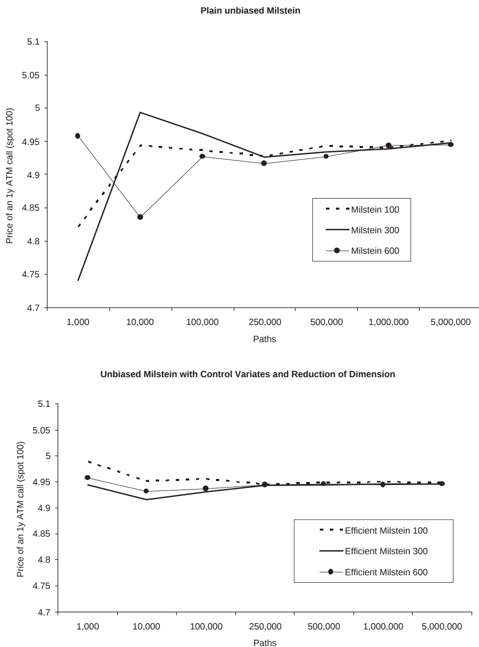
Figure 7.6: Comparison of the plain unbiased Milstein scheme to compute a European call price with the method discussed in section 7.2.4 for various steps per year. In particular, we see that the prices computed with this method are already relatively close to the true value for a very low number of paths.
