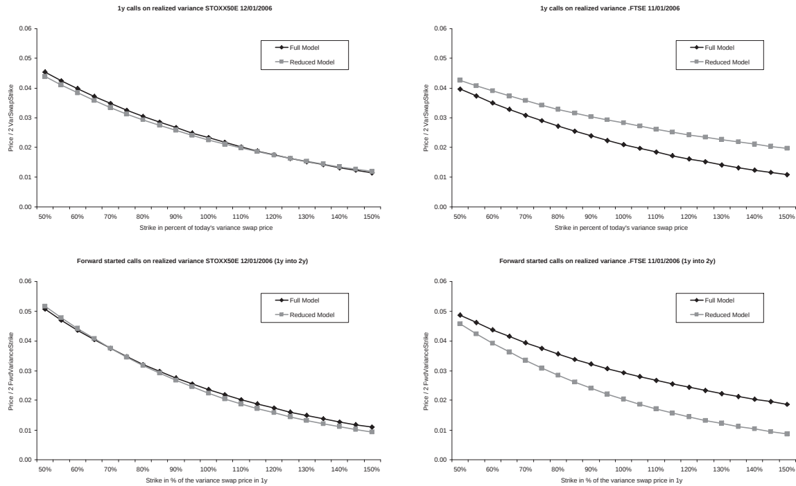
Figure 8.8: Calls on realized variance with one year maturity and forward started calls on realized variance for one year into two years. We find that if the models coincide for the spot started options, then they usually also give similar prices for the forward started version. This is in stark contrast to the prices for options on variance swaps, cf. figure 8.9.
