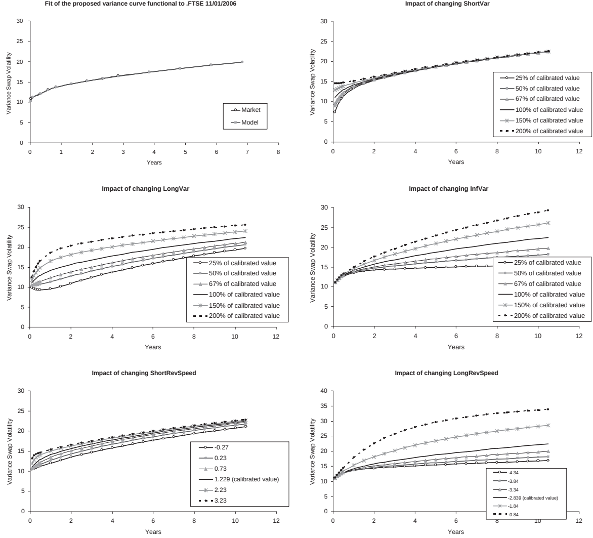
Figure 7.3: The impact of changes of the parameters to the curve calibrated to FTSE market data on January 11th, 2006; the top left graph recalls the fit to the market. The calibrated values for the FTSE are given in table 8.1 on page 138.
