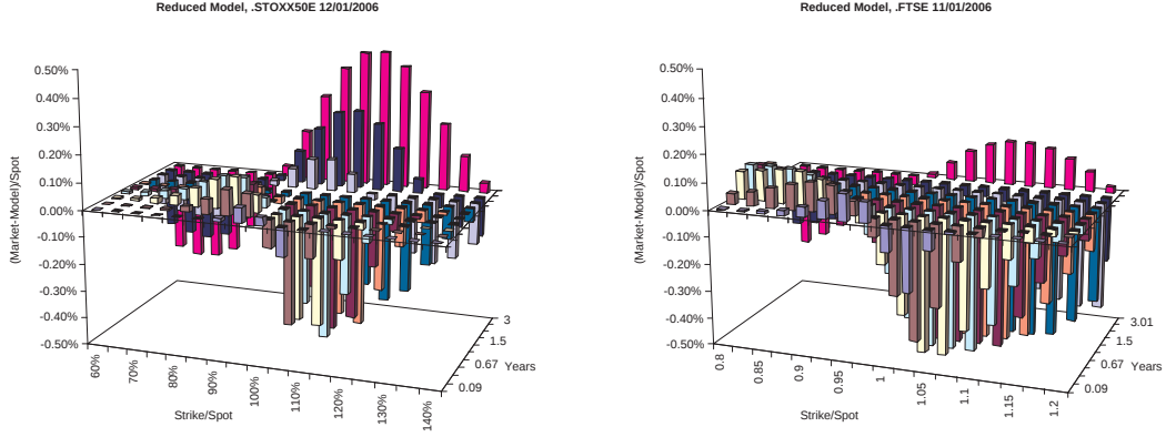
Figure 8.3: Calibration of the reduced model (8.24) to STOXX50E and FTSE market data.
