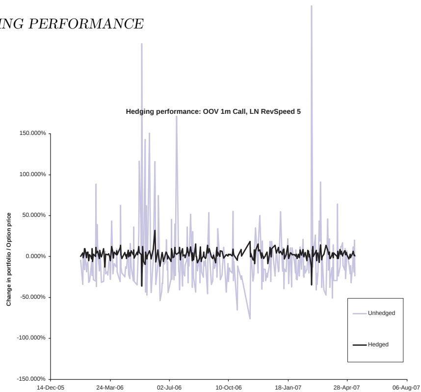
Figure 4.7: Hedging a 1m ATM call on variance with Fitted LN. Standard deviation is 42% for the unhedged position and 6% for the hedged position.
