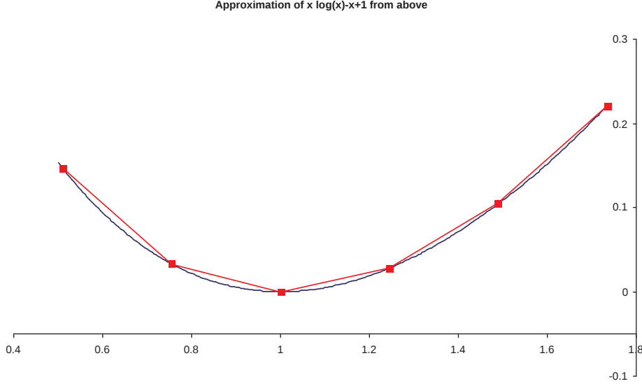
Figure A.3: Approximation of G(x, K^*) := x \log(x/K^*) - x + K^* from above. Note the striking similarity to figure A.2.
