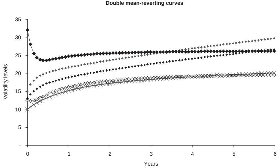
Figure 3.1: Various shapes of the variance swap prices given for various parameterizations of the functional (3.7). The graph shows “variance swap volatilities” \sqrt{\int_0^T G(z; x) dx/T} , cf. (1.2).
