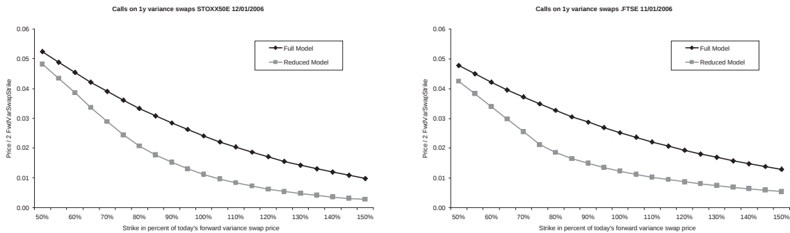
Figure 8.9: Calls on a forward variance swap according to (8.25). Note the difference in the option prices even for STOX50E, for which the spot started and forward started options are very similar. The difference in prices for options on variance swaps in the two models is due to the fact that the full model allows more variation in the term structure of variance swaps, as can also be seen by comparing figures 8.5 and 8.6. This highlights the importance of the use of multi-factor models for pricing term-structure deals. See also figure 8.10.
