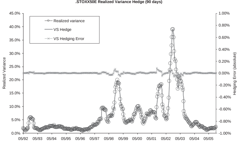
Figure A.1: Realized variance versus its hedge (A.4).
