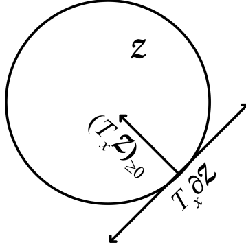
Figure 2.1: The tangent spaces (\mathcal{T}_x \mathcal{Z})_{\geq 0} and \mathcal{T}_x \partial \mathcal{Z} for a point x \in \partial \mathcal{Z} .
