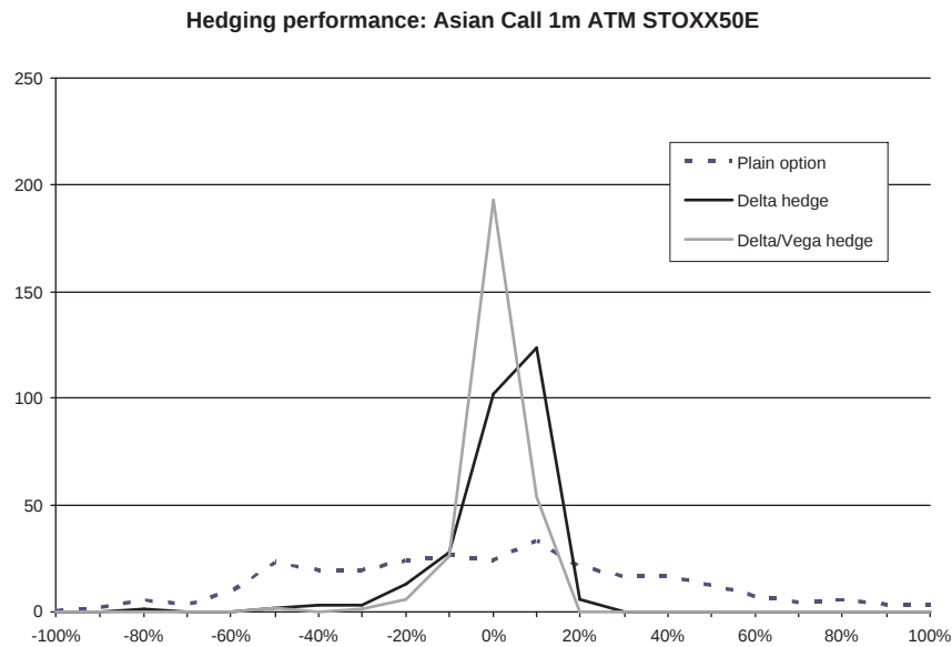
Figure 4.5: Histogram of hedging an Asian option with Black&Scholes. The reduction of risk in the P&L is clearly visible.
