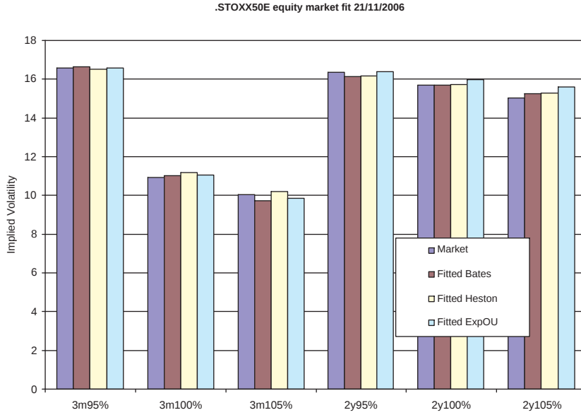
Figure 4.1: The result of calibrating Fitted Heston, Fitted Bates and Fitted Exponential Ornstein-Uhlenbeck to .STOXX50E vanilla options on equity.
