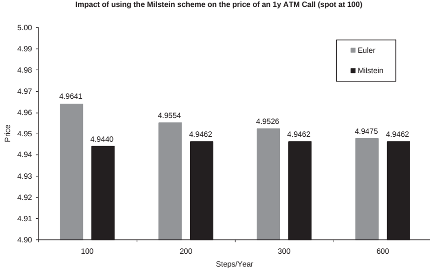
Figure 7.4: The price of an 1y ATM call with Euler and Milstein, respectively. We can clearly see the improved convergence with the Milstein scheme.
